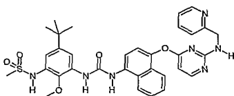
N-{5-tert-Butyl-2-methoxy-3-[3-(4-{2-[(pyridin-2-ylmethyl)-amino]-pyrimidin-4-yloxy}-naphthalen-1-yl)-ureido]-phenyl}-methanesulfonamide;
